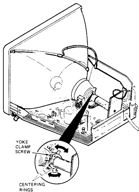
Figure 3-2 Rotation and Centering Adjustments
