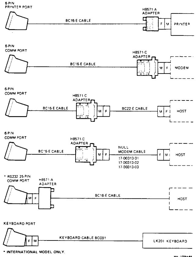
Figure A-1 VT320 Cables
