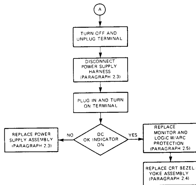
Figure 1-2 VT320 Troubleshooting Flowchart
