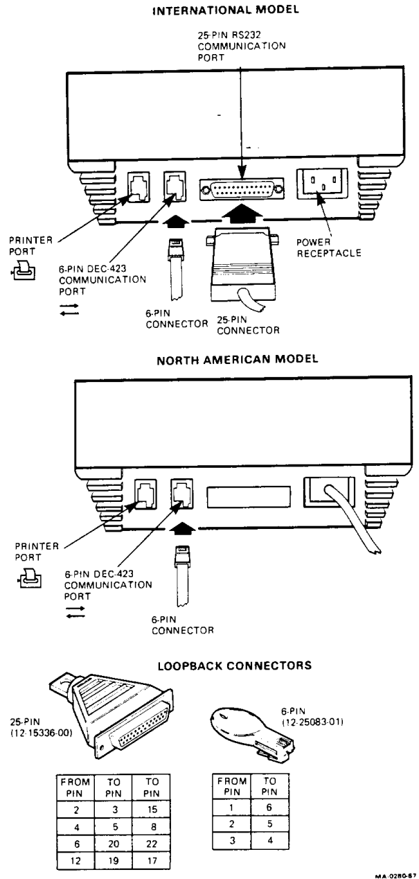
Figure 1-4 VT320 Rear Connector Panel and Loopback Connectors
